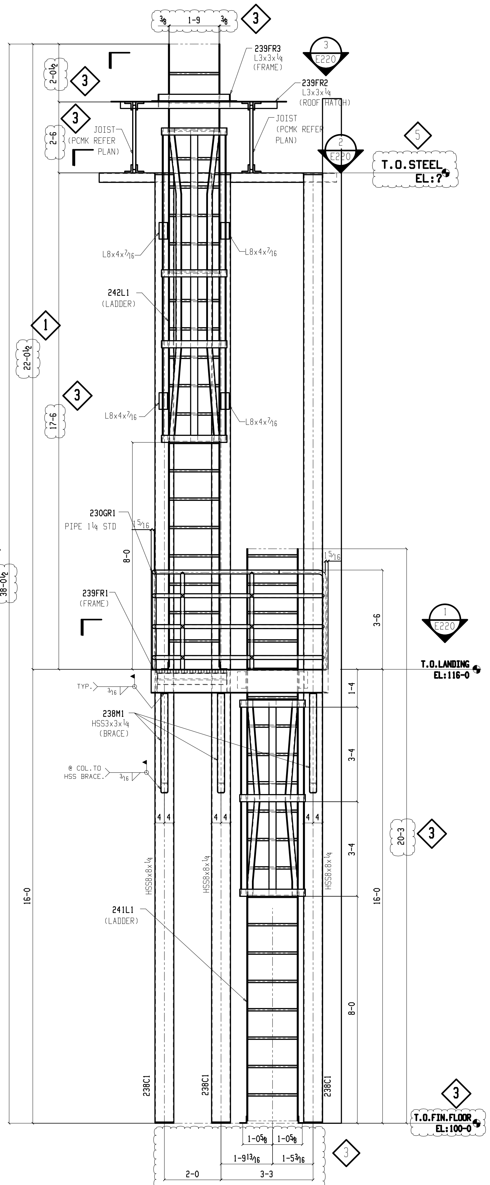
CAGE LADDER BUILDING #B (REF DWG NO: 1/AB.03)
