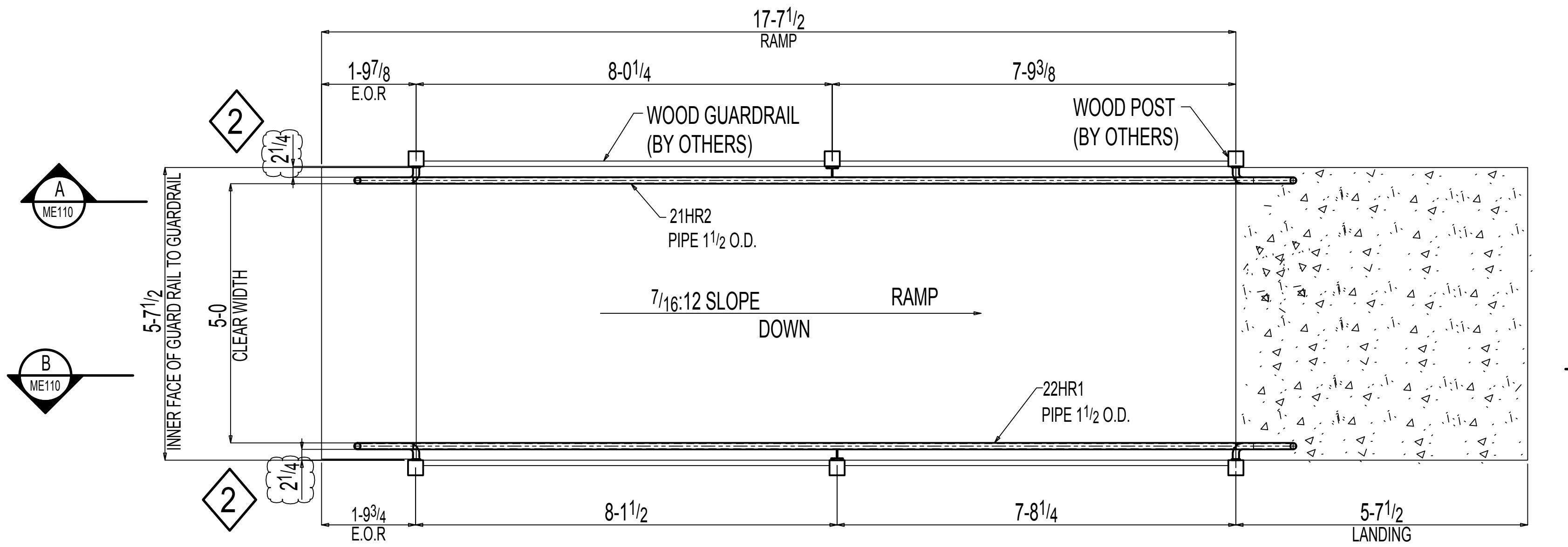
DETAIL-1 ME110 REF: 1/A2.01
