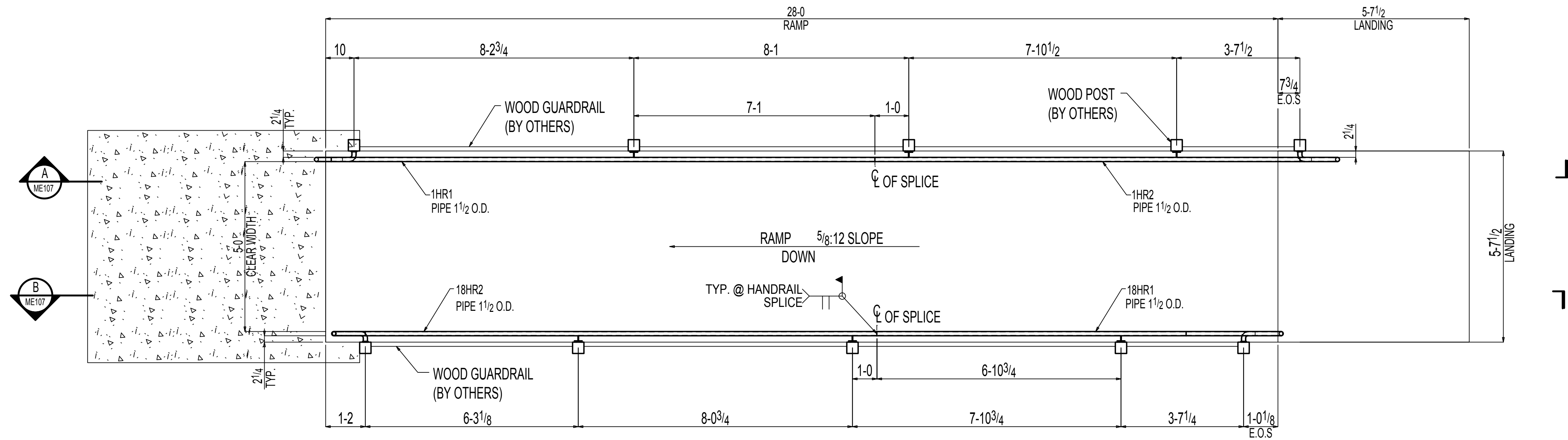
DETAIL-1 ME106 REF: 3/A2.01
