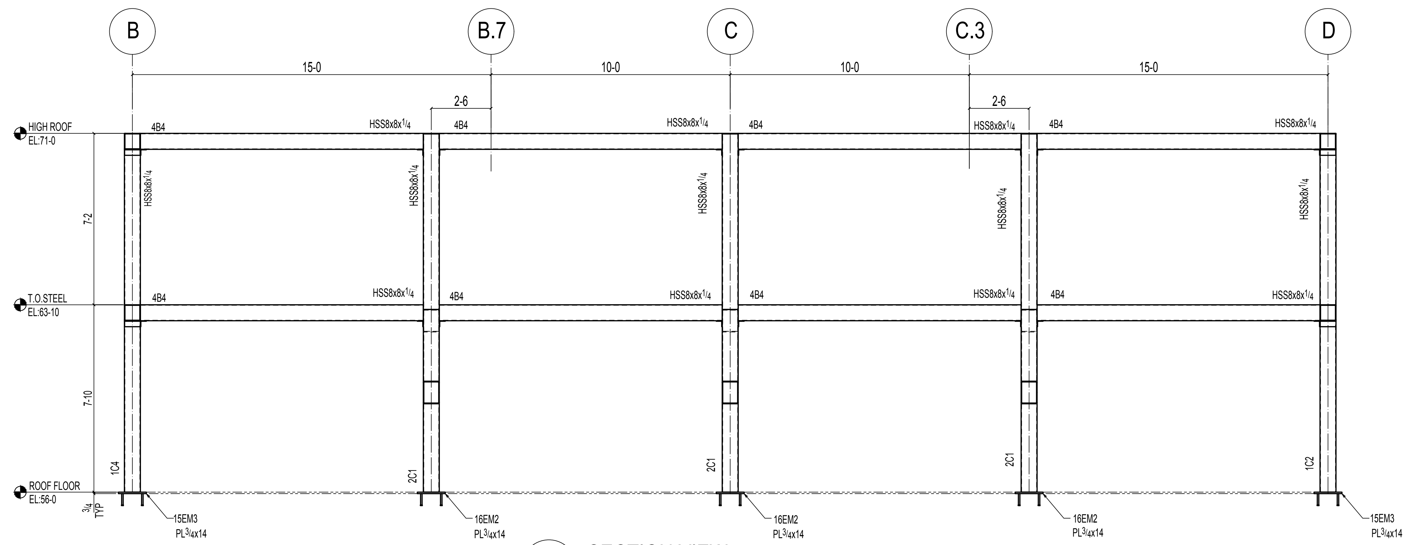
C SECTION VIEW E5 (REF:3/S4.501)
