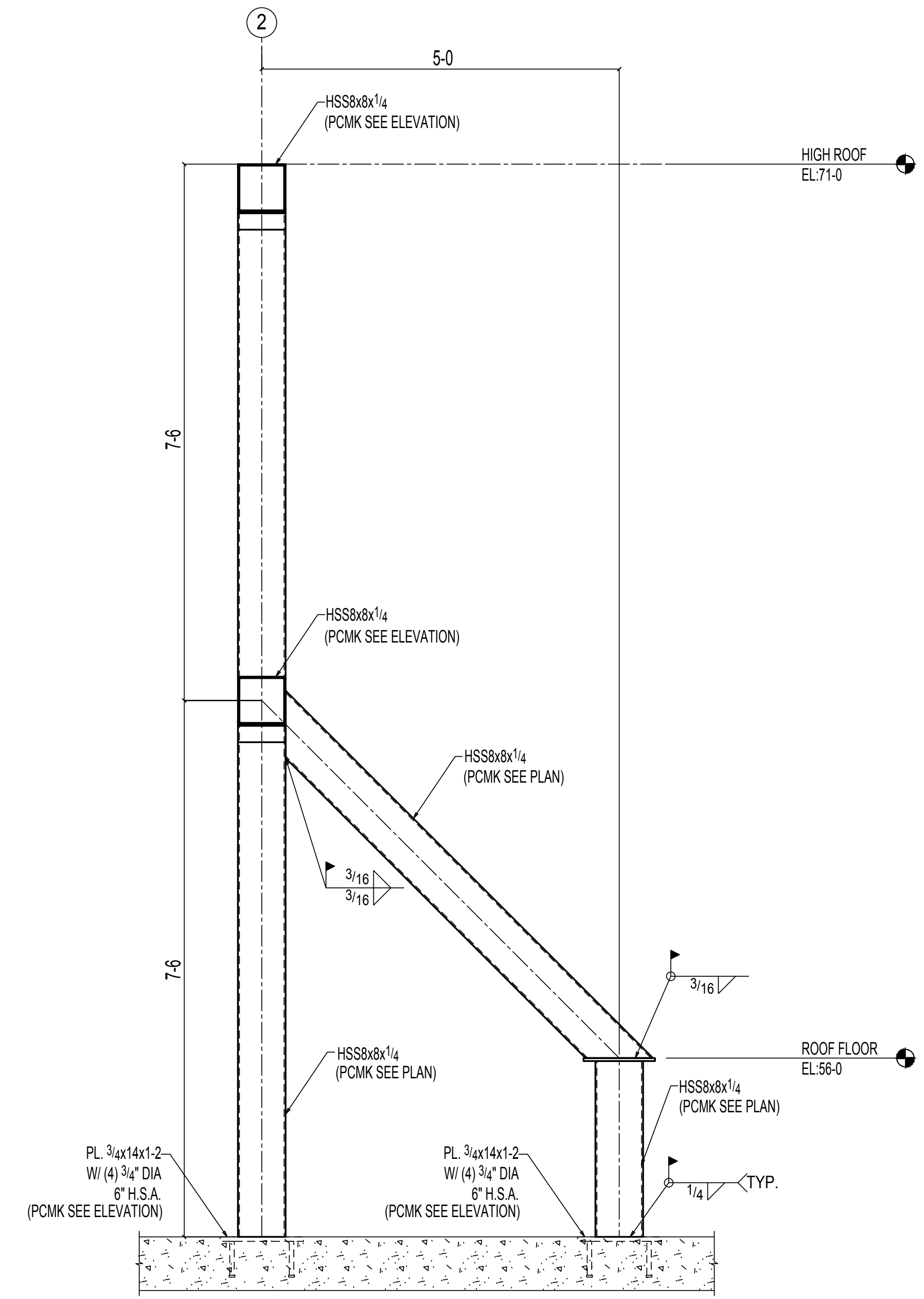
A SECTION VIEW E2 (REF:2/S4.401)
