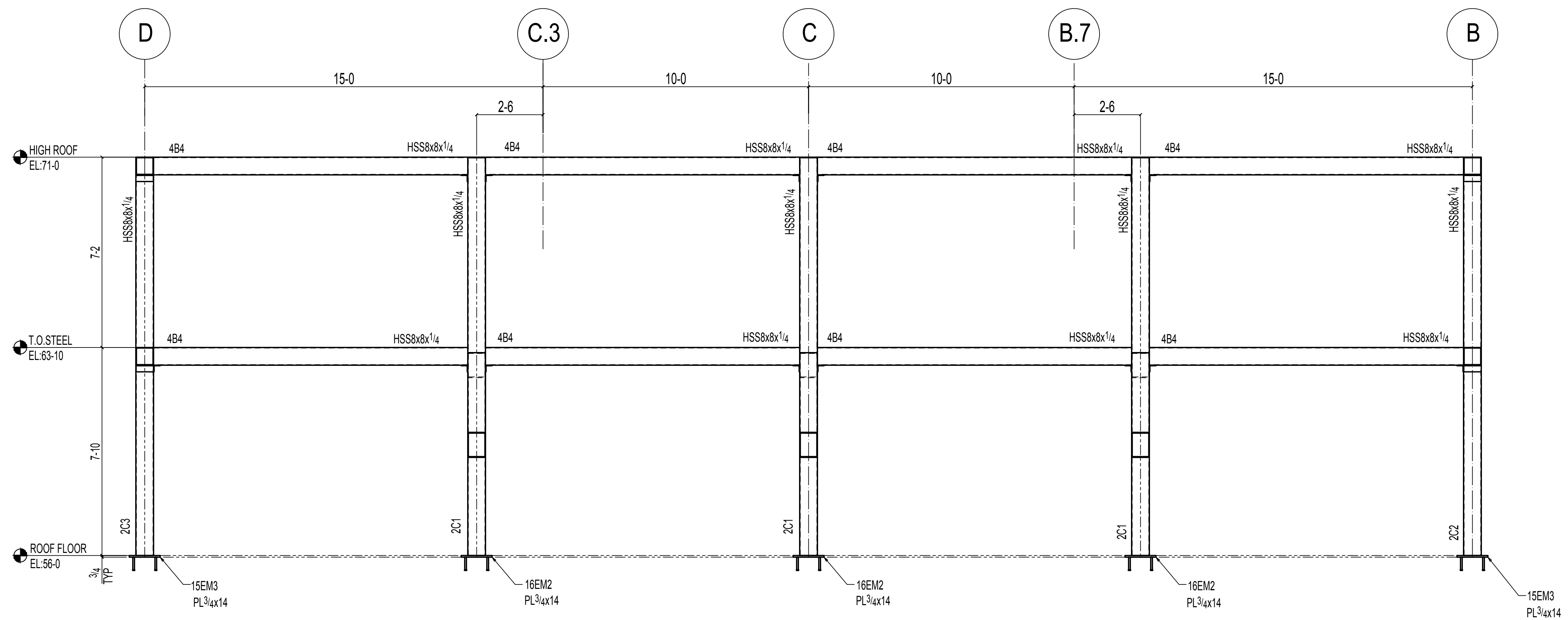
B SECTION VIEW E5 (REF:4/S4.501)
