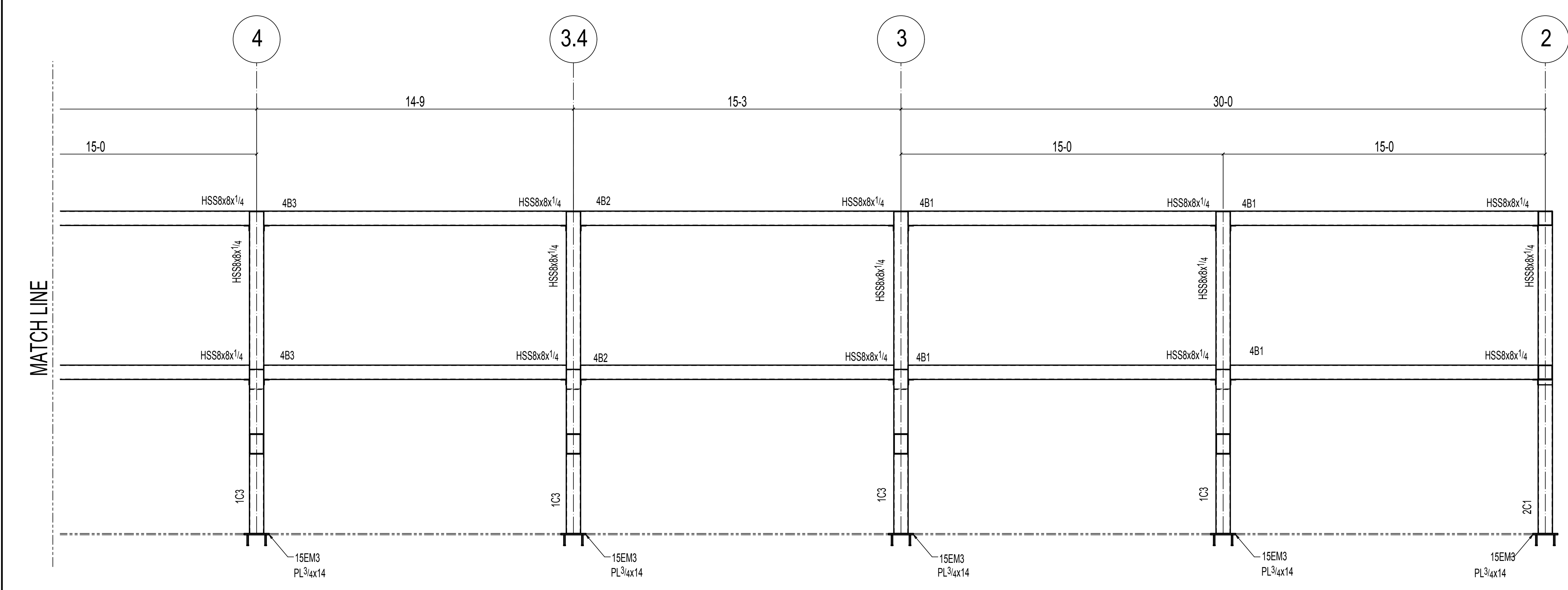
A SECTION VIEW E6 (REF: 2/S4.501)
