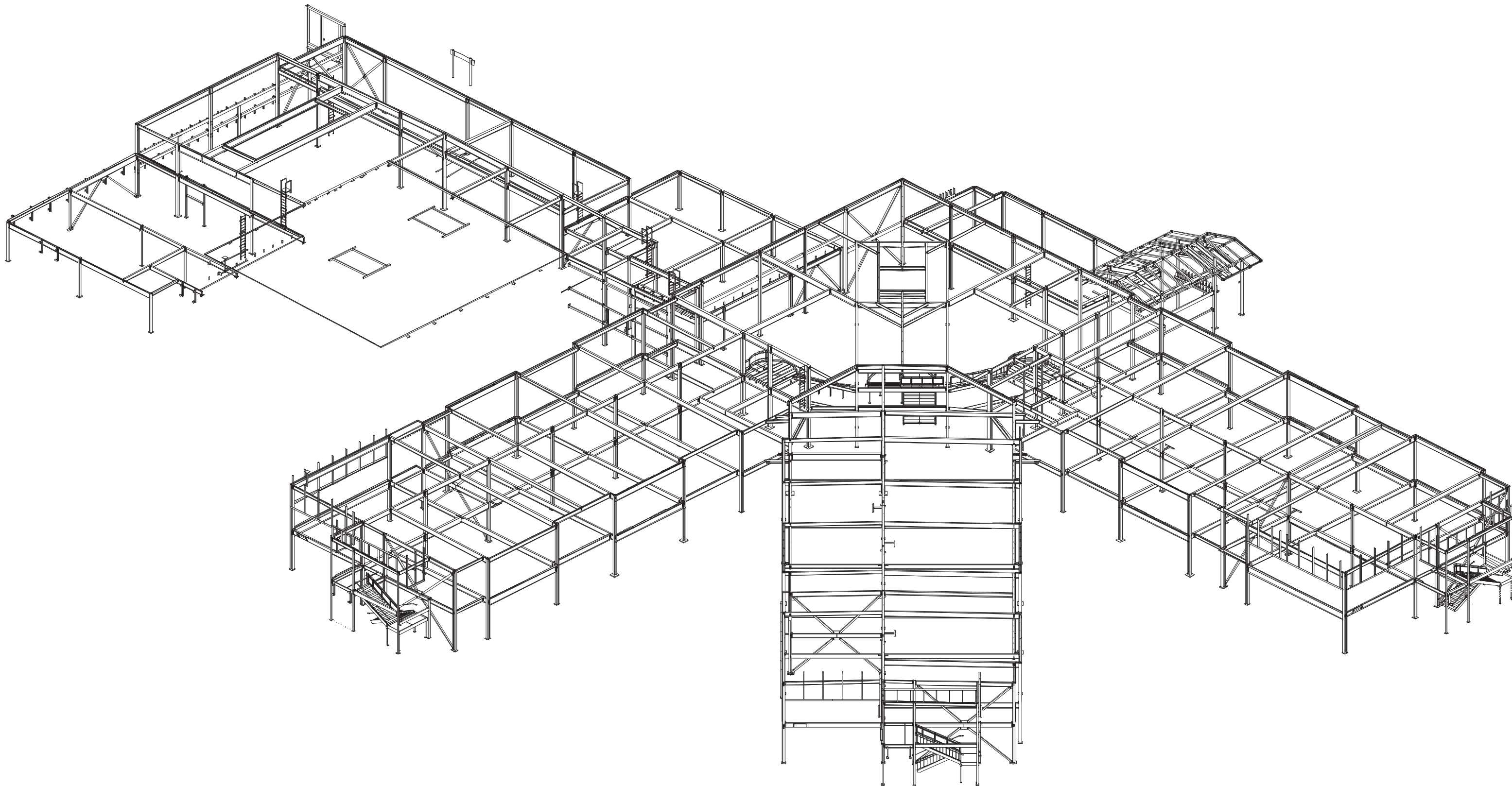
ISOMETRIC VIEW
